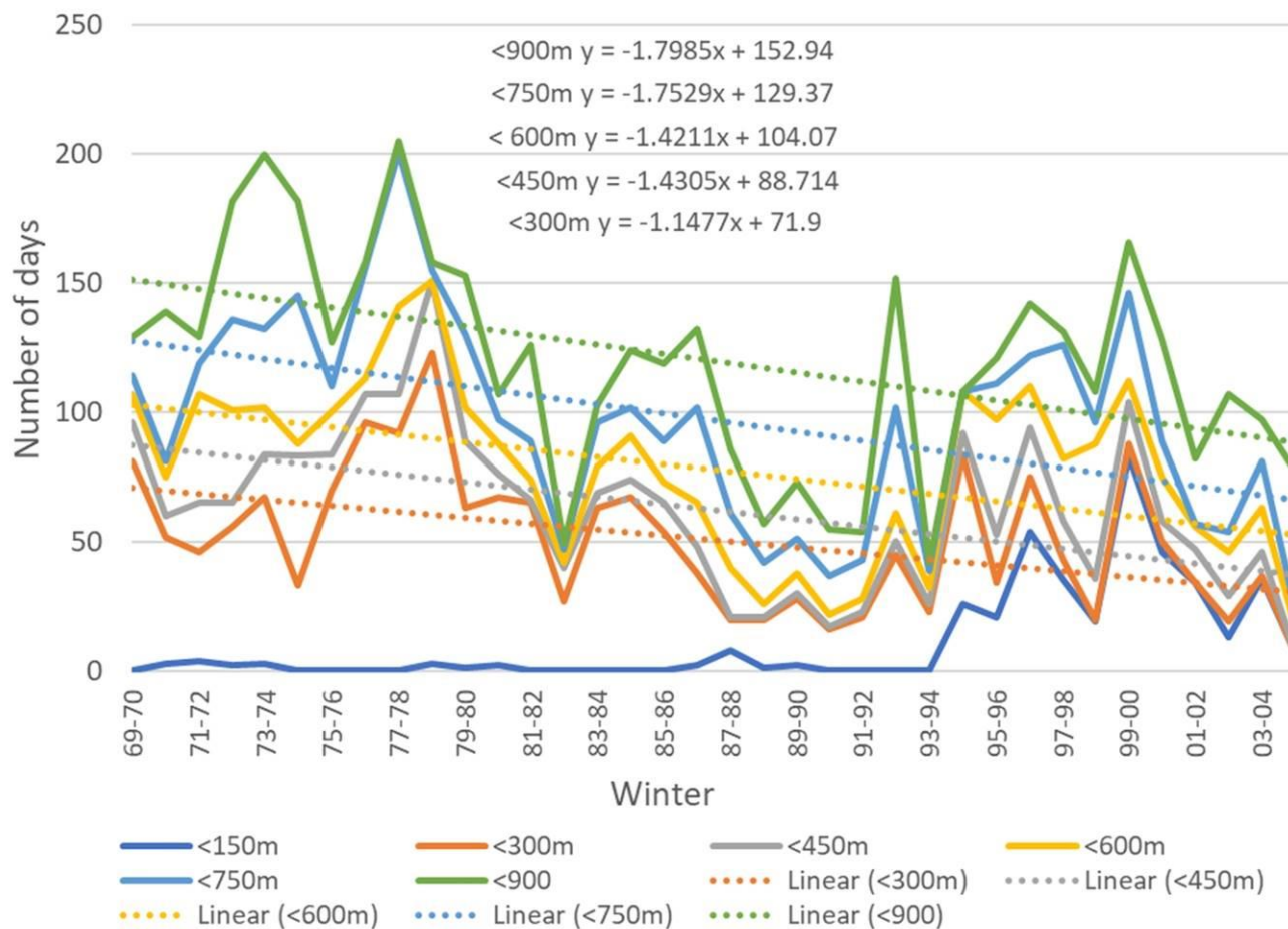
Figure 2: Number of days per year of snow cover at or below specific elevations and estimated trends for Whitehillochs between 1969 and 2005.
