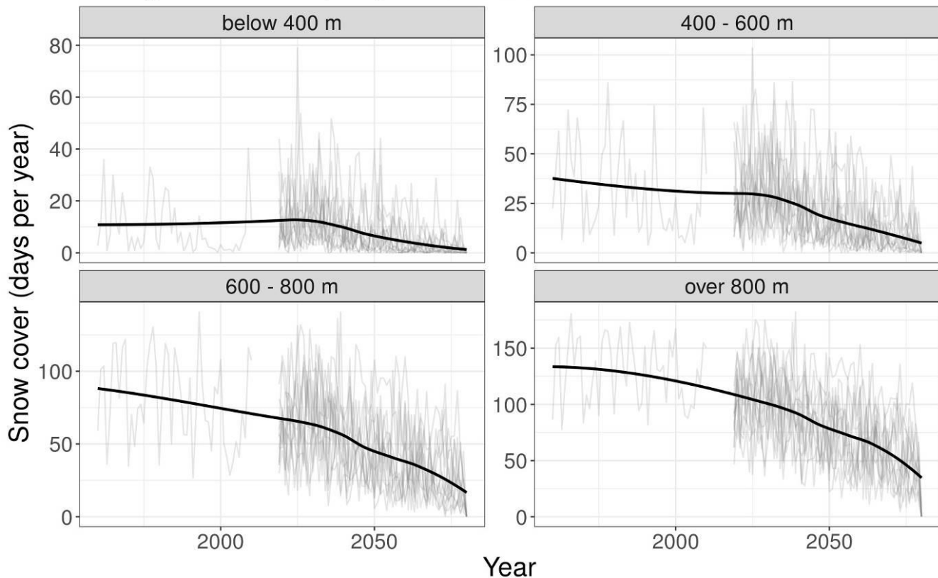
Figure 5: Annual snow cover (days per year) at four elevation ranges for the Cairngorms National Park. Light grey lines show individual model runs with the heavy black line indicating the smoothed average of these.
