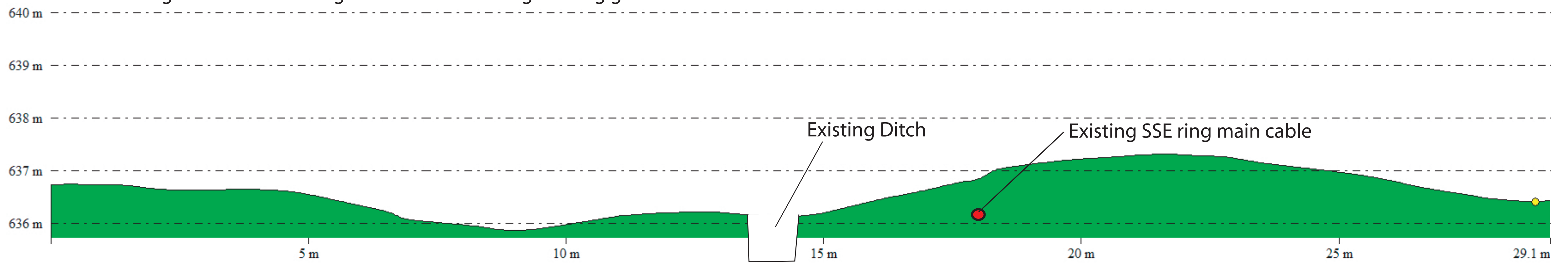
Section through AREAS BCH Along section line showing existing ground level.
