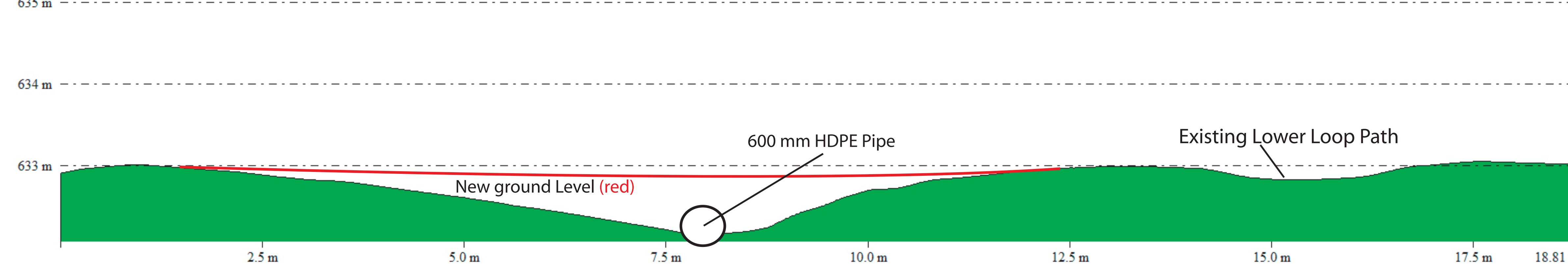
Section through AREA A showing new ground level.
