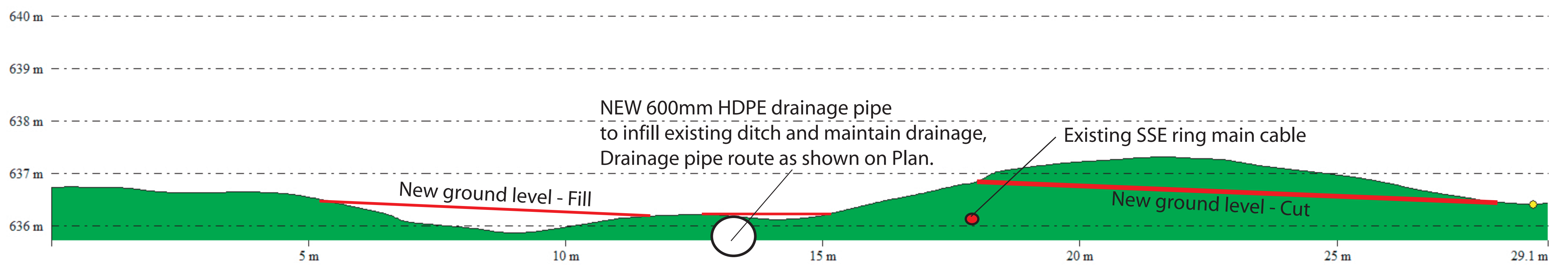
Section through AREAS BCH Along section line showing New ground level.
