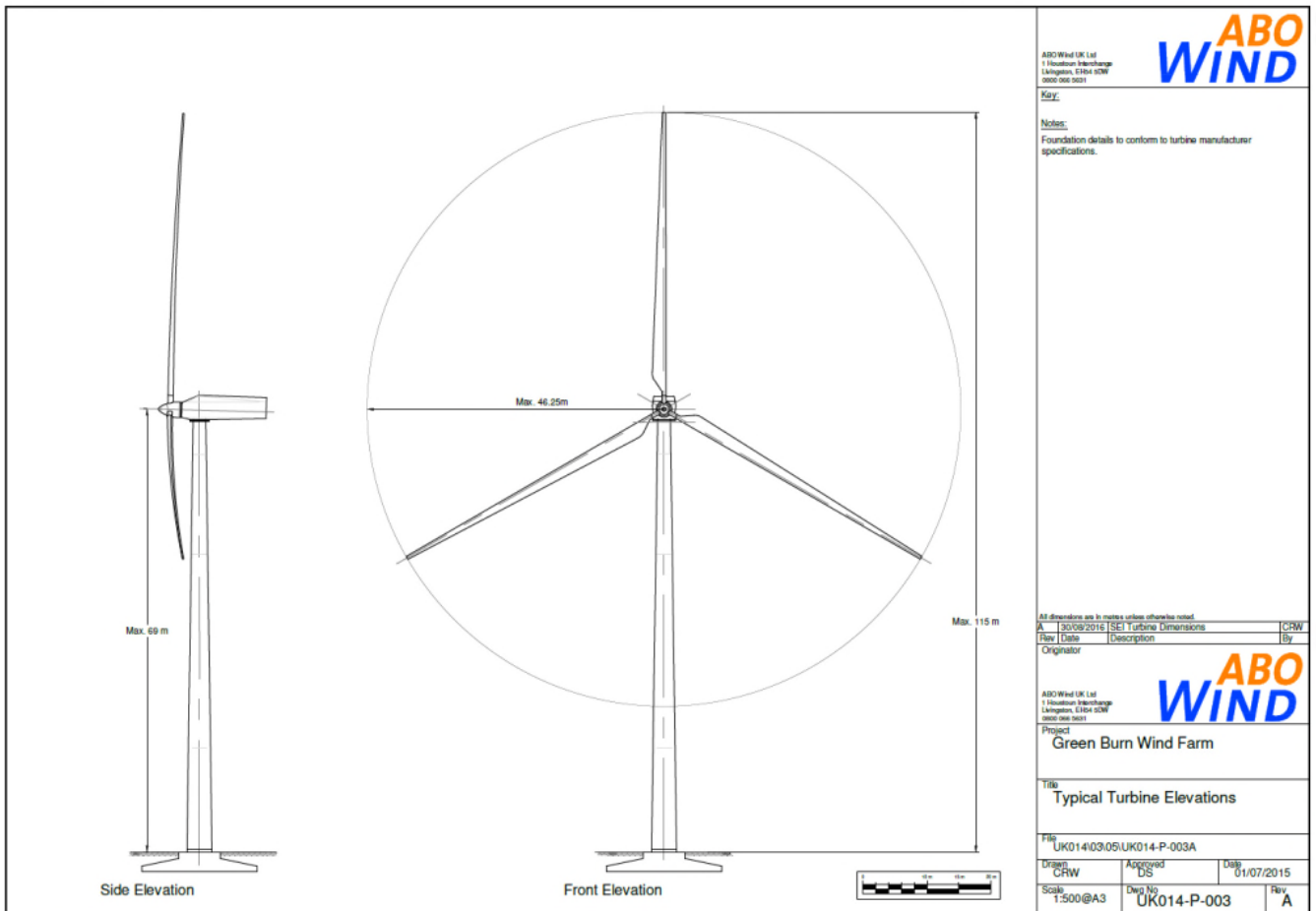
Appendix 2 Revised Site Plan and Turbine Elevations
