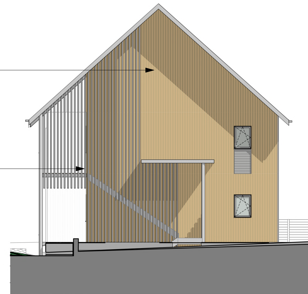
E08 Block B East Elevation 1:100
