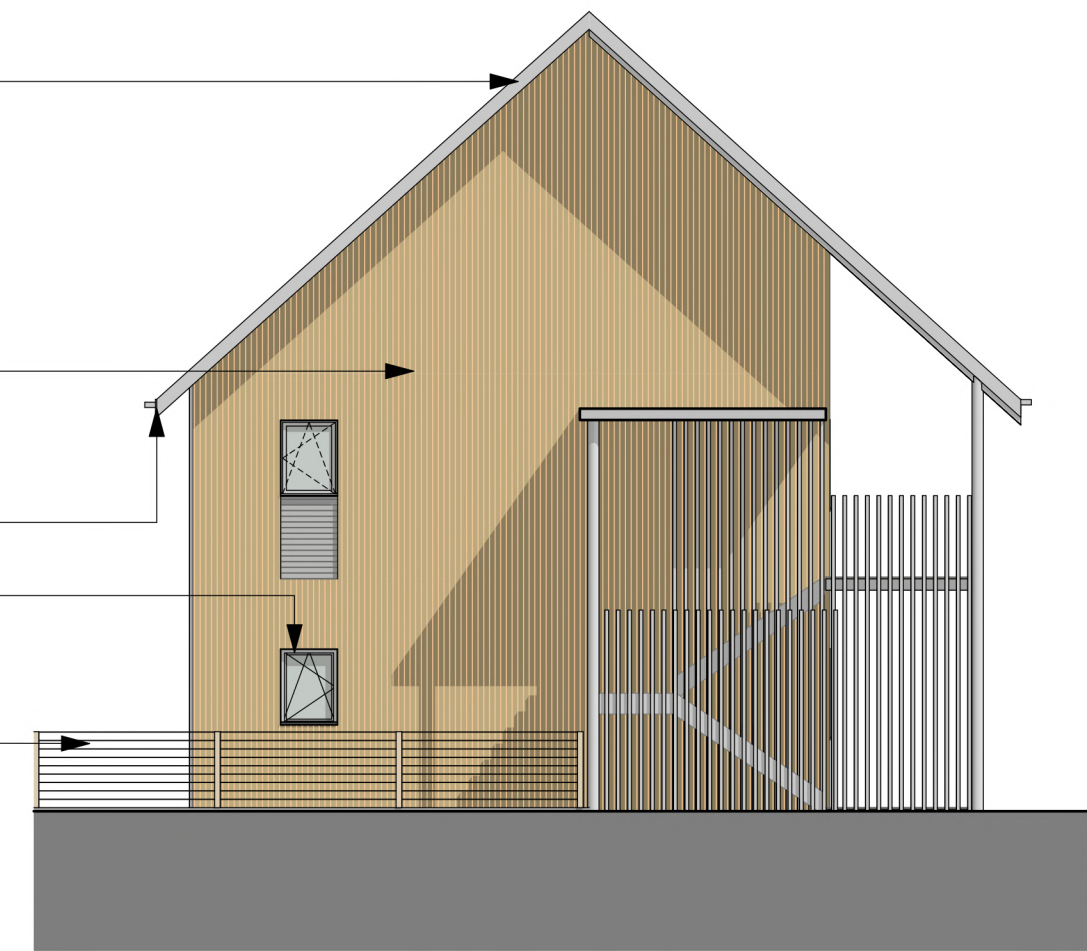
E06 Block B West Elevation 1:100
