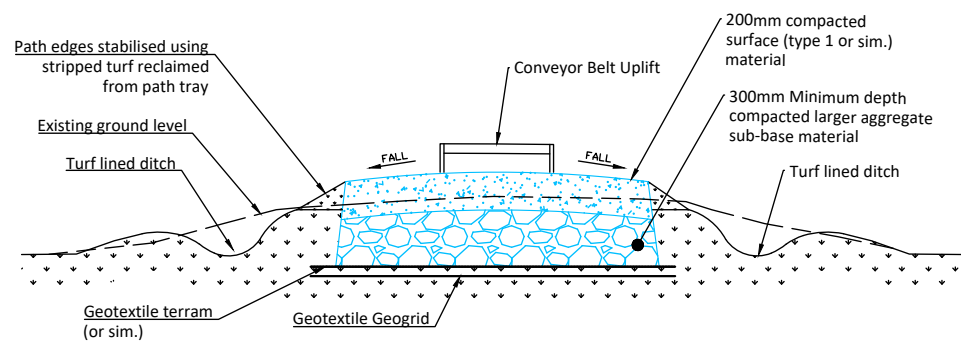
Conveyor Belt Track Construction Detail
