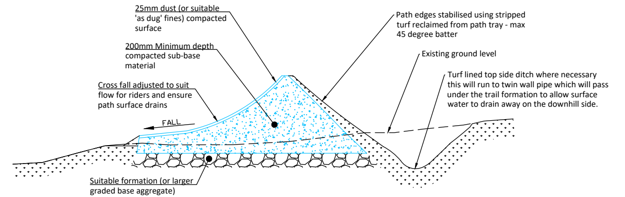
Typical 'Berm' Trail Construction Detail
