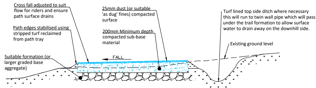
Typical Trail Construction Detail
