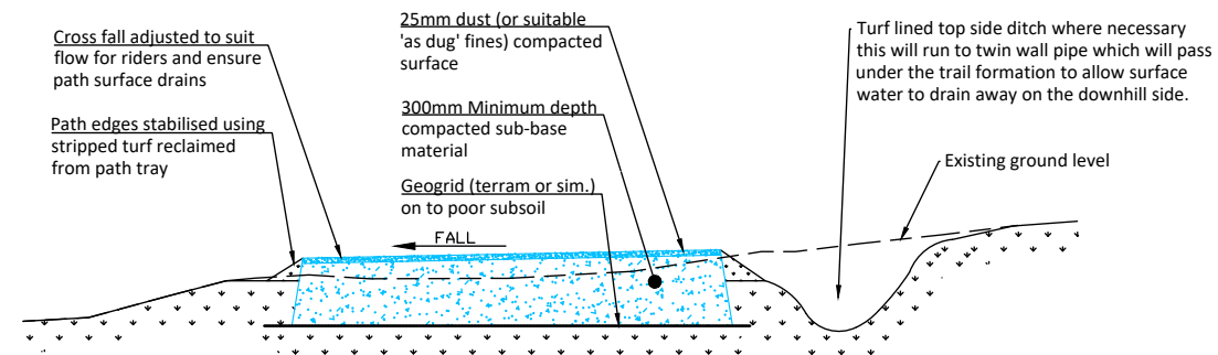
Floated Trail Construction Detail
