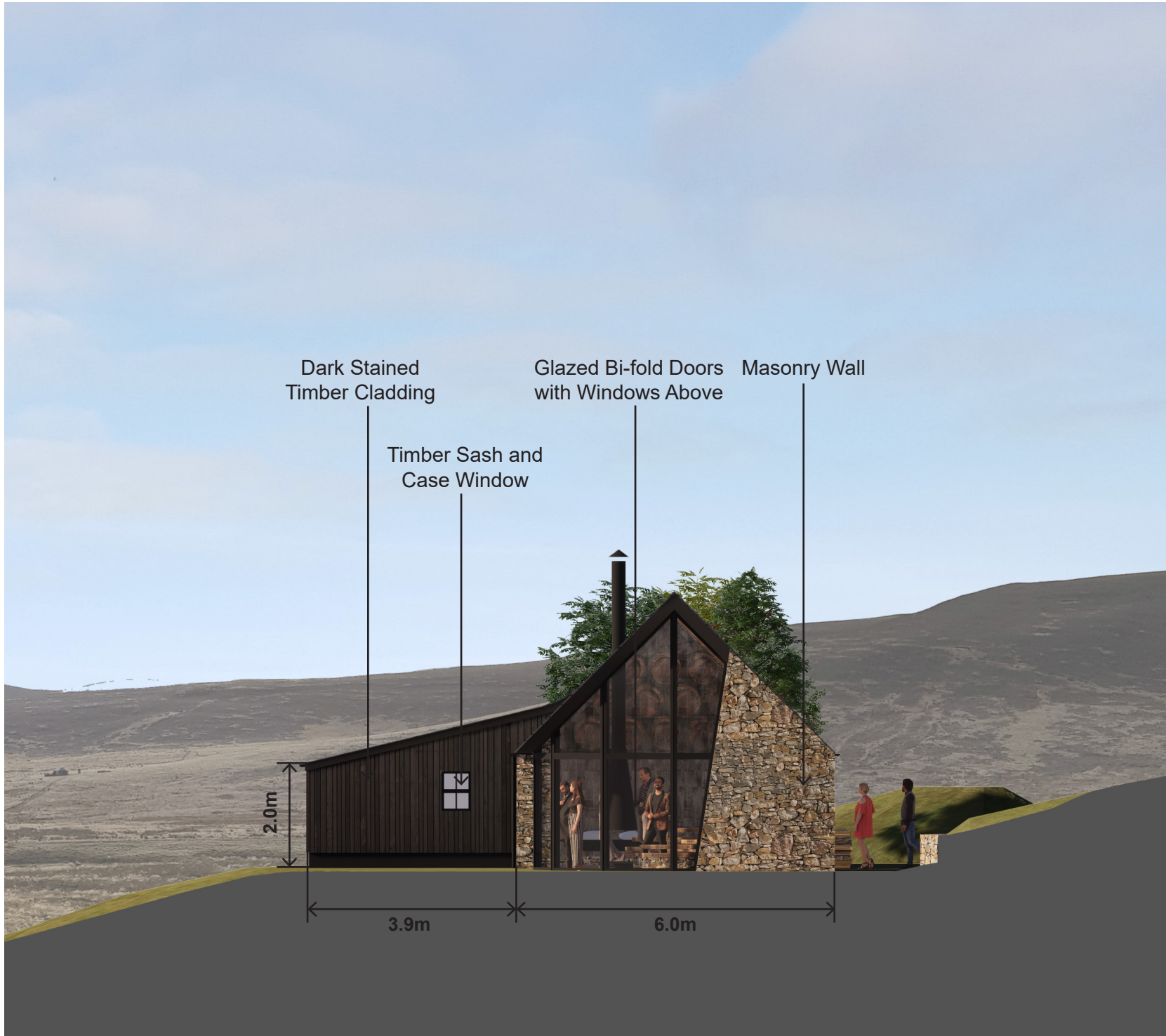
North Elevation - Scale 1:100
