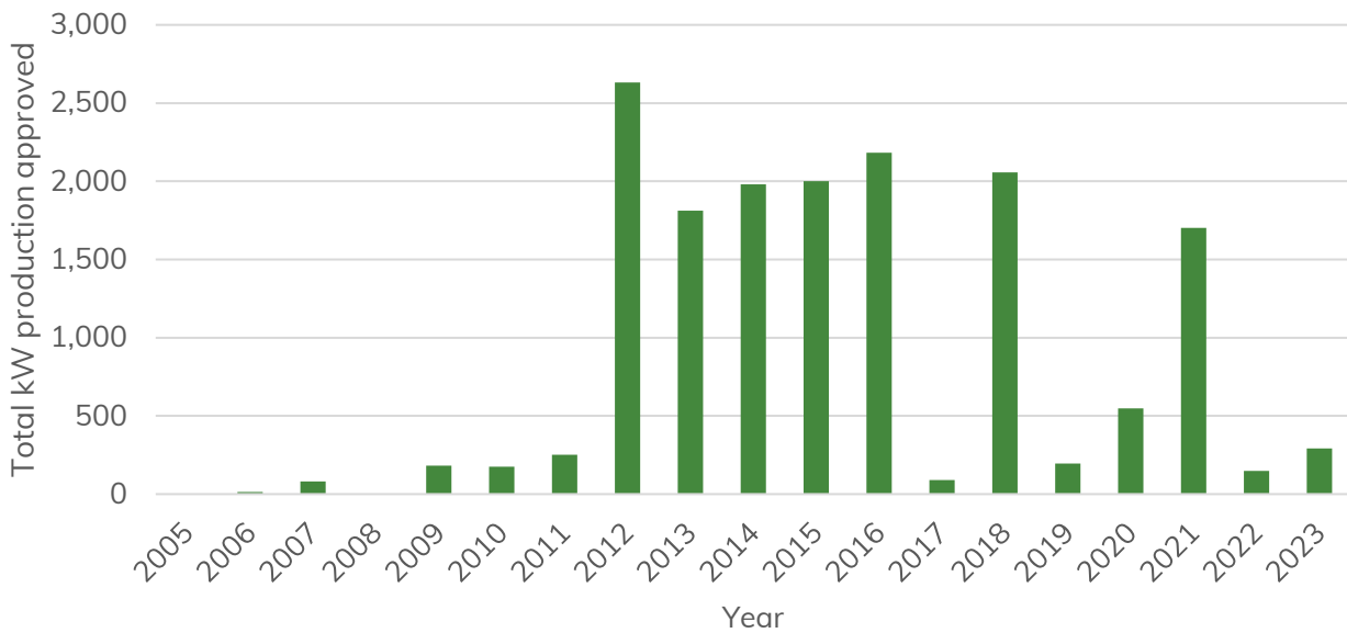
Figure 8 The total annual kW of installed renewable energy generation delivered through planning permissions in the National Park, 2005 – 2023 (Data available through planning applications submitted to Cairngorms National Park Authority and local authorities).
