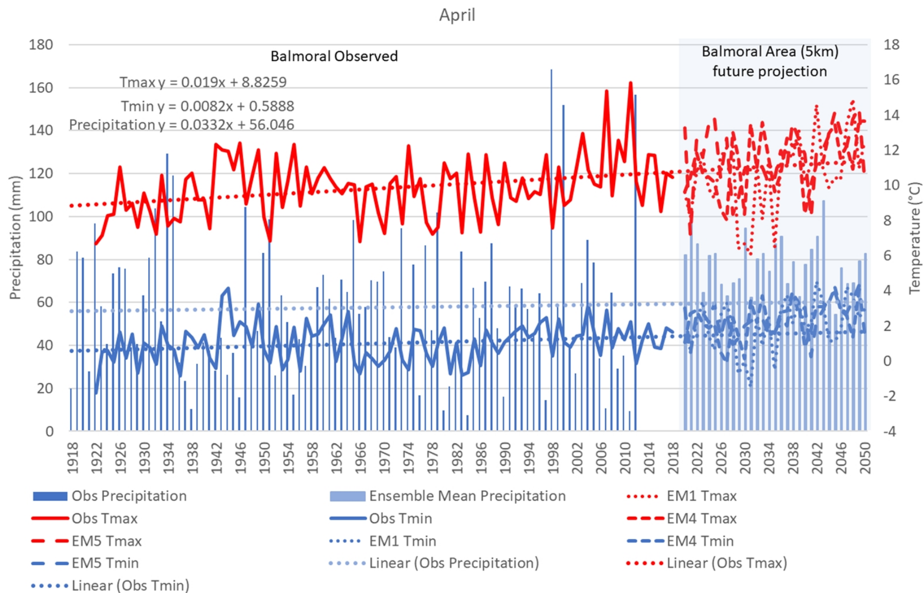
Figure 11: Weather data trends for April, Balmoral 1918-2018 and estimated future 2020-2050 (RCP8.5)
