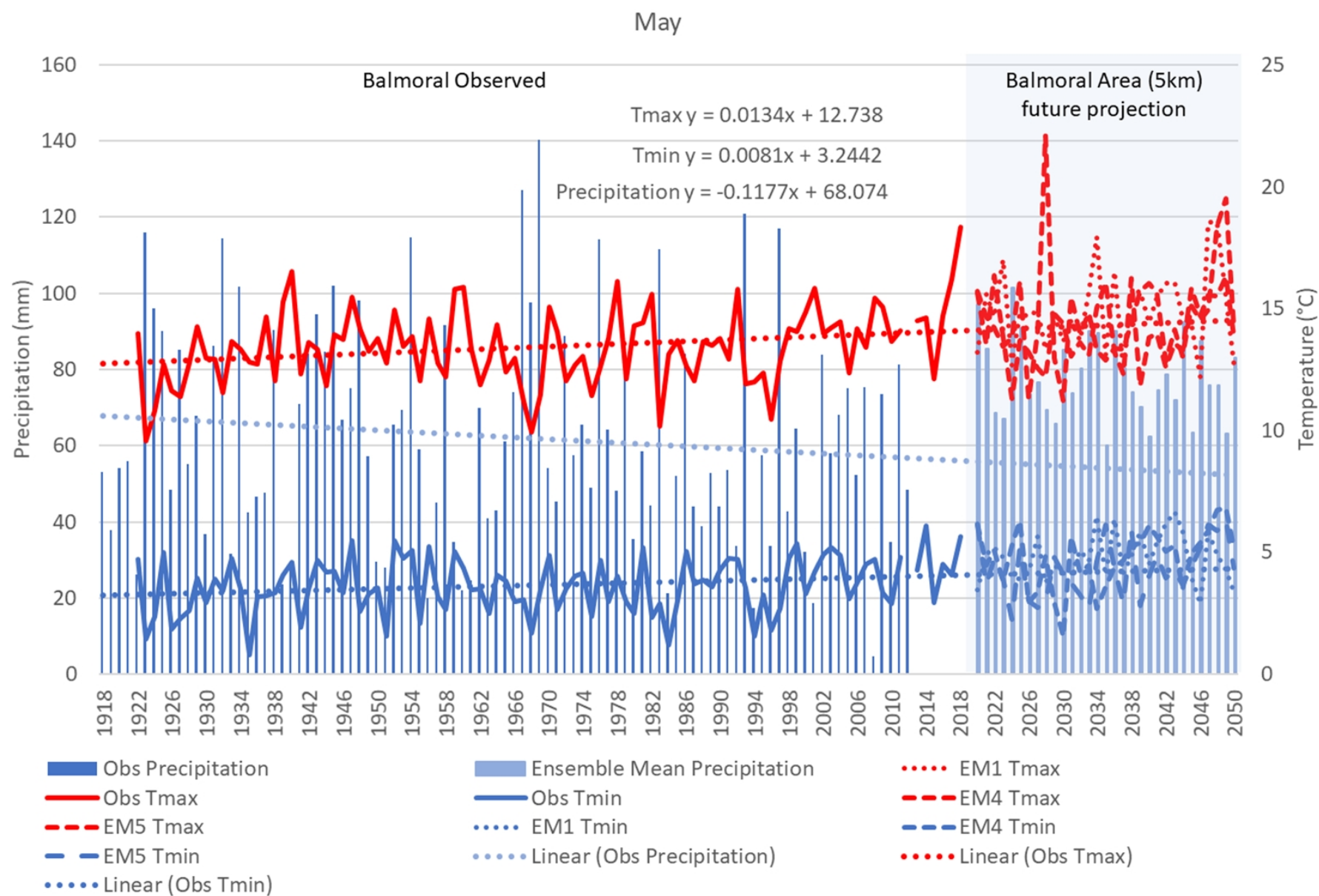
Figure 12: Weather data trends for May, Balmoral 1918-2018 and estimated future 2020-2050 (RCP8.5)
