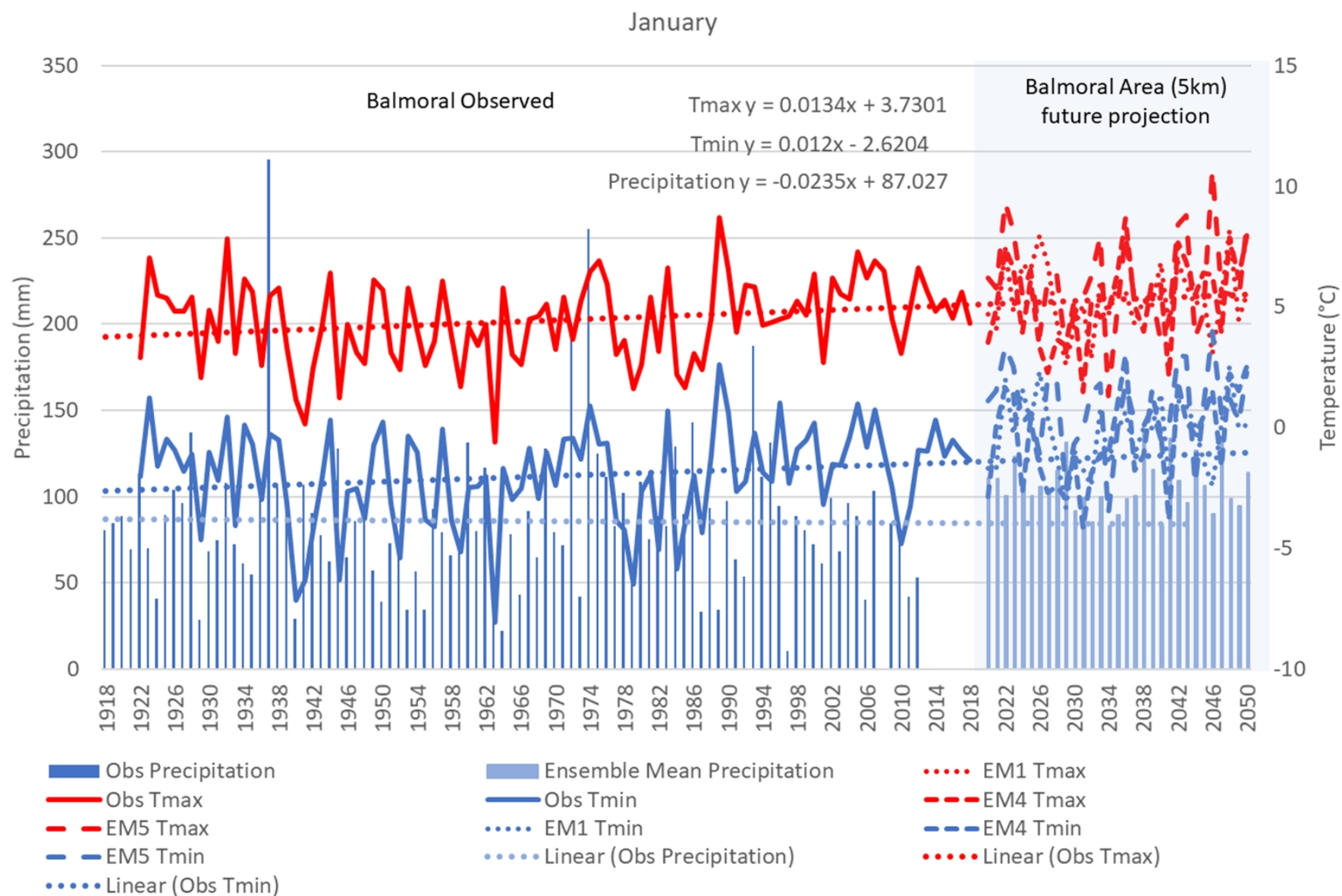
Figure 8: Weather data trends for January, Balmoral 1918-2018 and estimated future 2020-2050 (RCP8.5)
