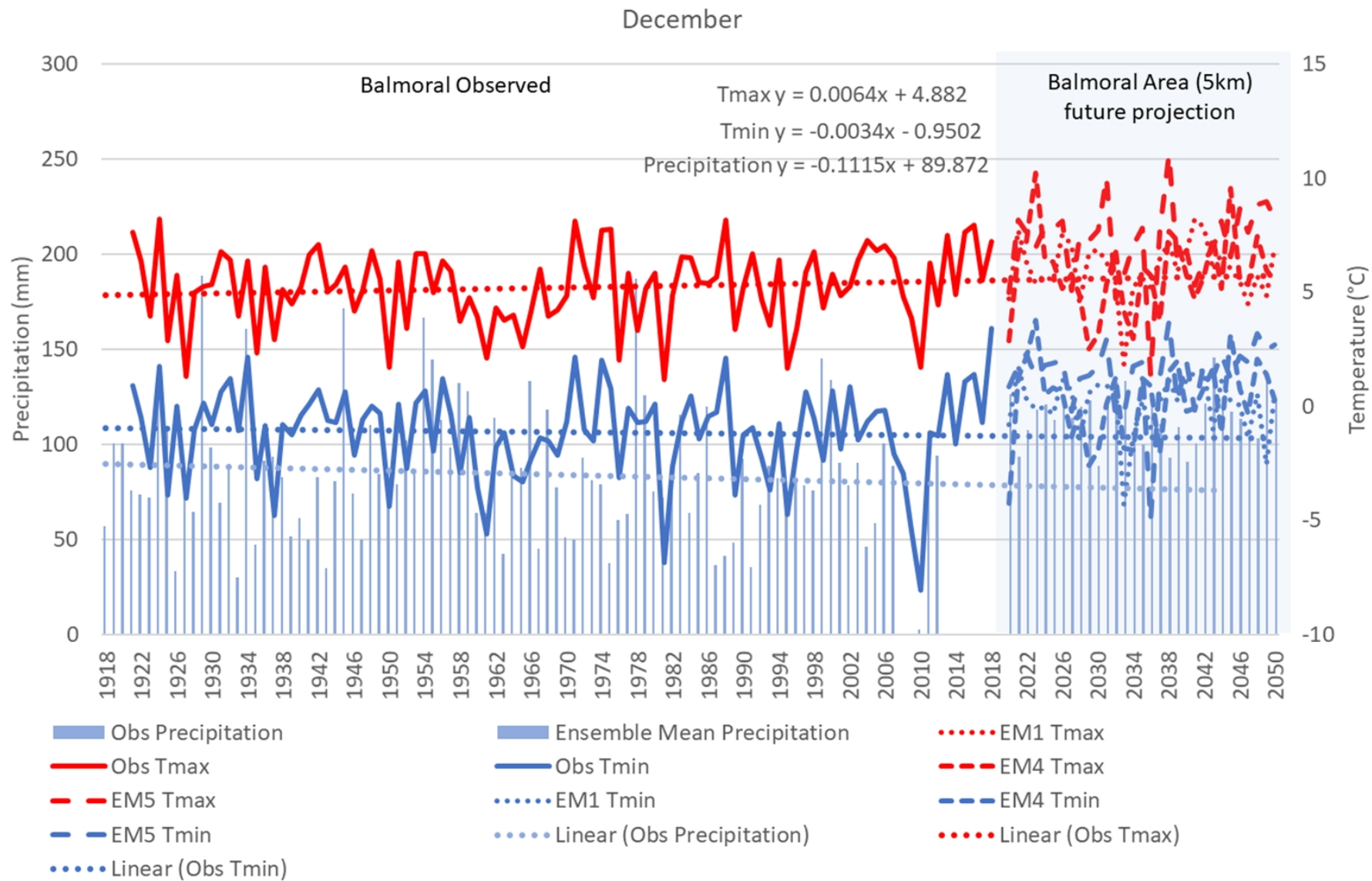
Figure 7: Weather data trends for December, Balmoral 1918-2018 and estimated future 2020-2050 (RCP8.5)
