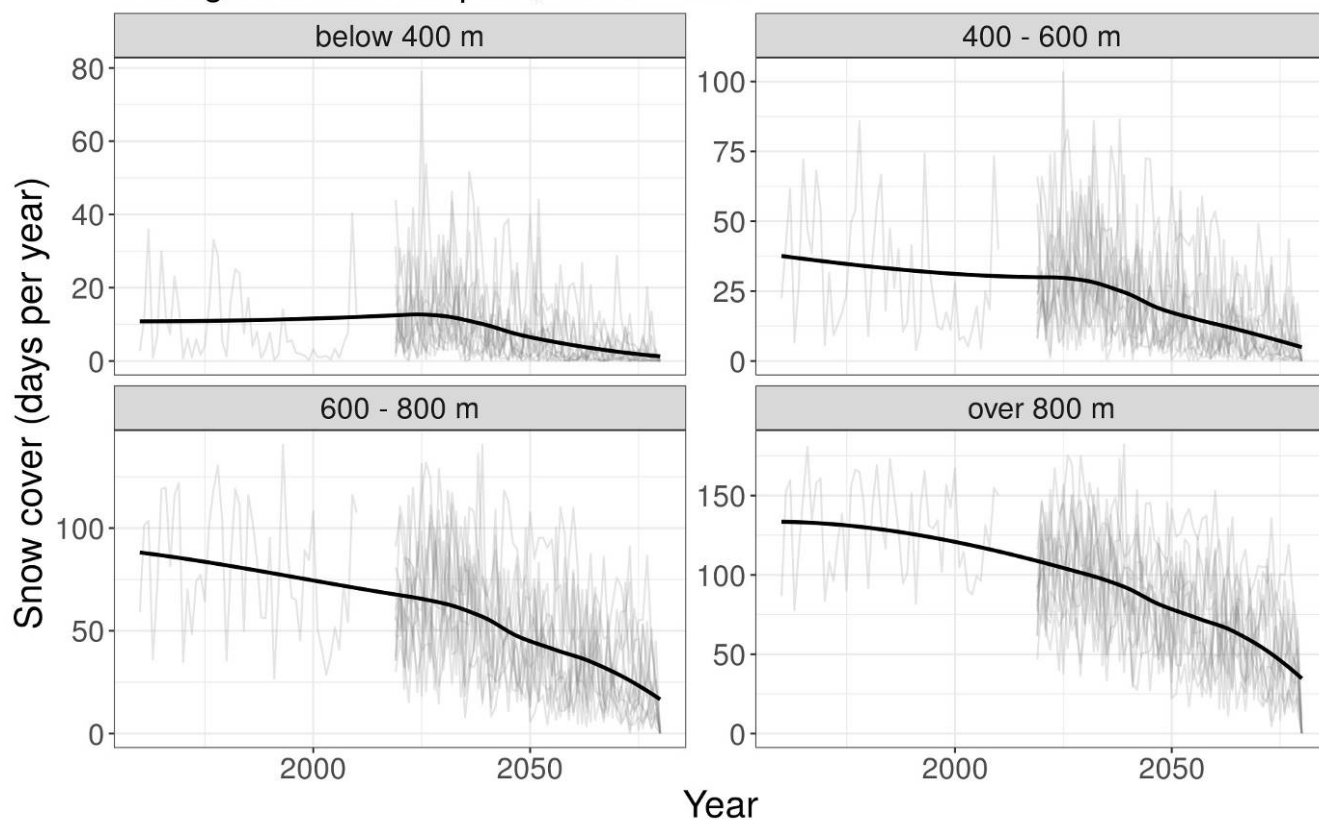
Figure 5: Annual snow cover (days per year) at four elevation ranges for the Cairngorms National Park. Light grey lines show individual model runs with the heavy black line indicating the smoothed average of these.
