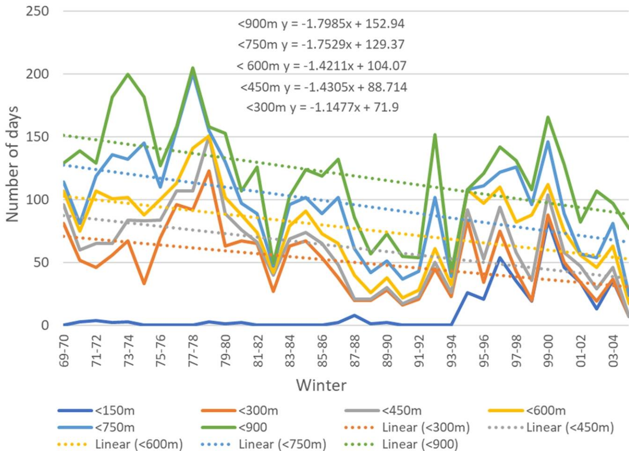
Figure 2: Number of days per year of snow cover at or below specific elevations and estimated trends for Whitehillocks between 1969 and 2005.
