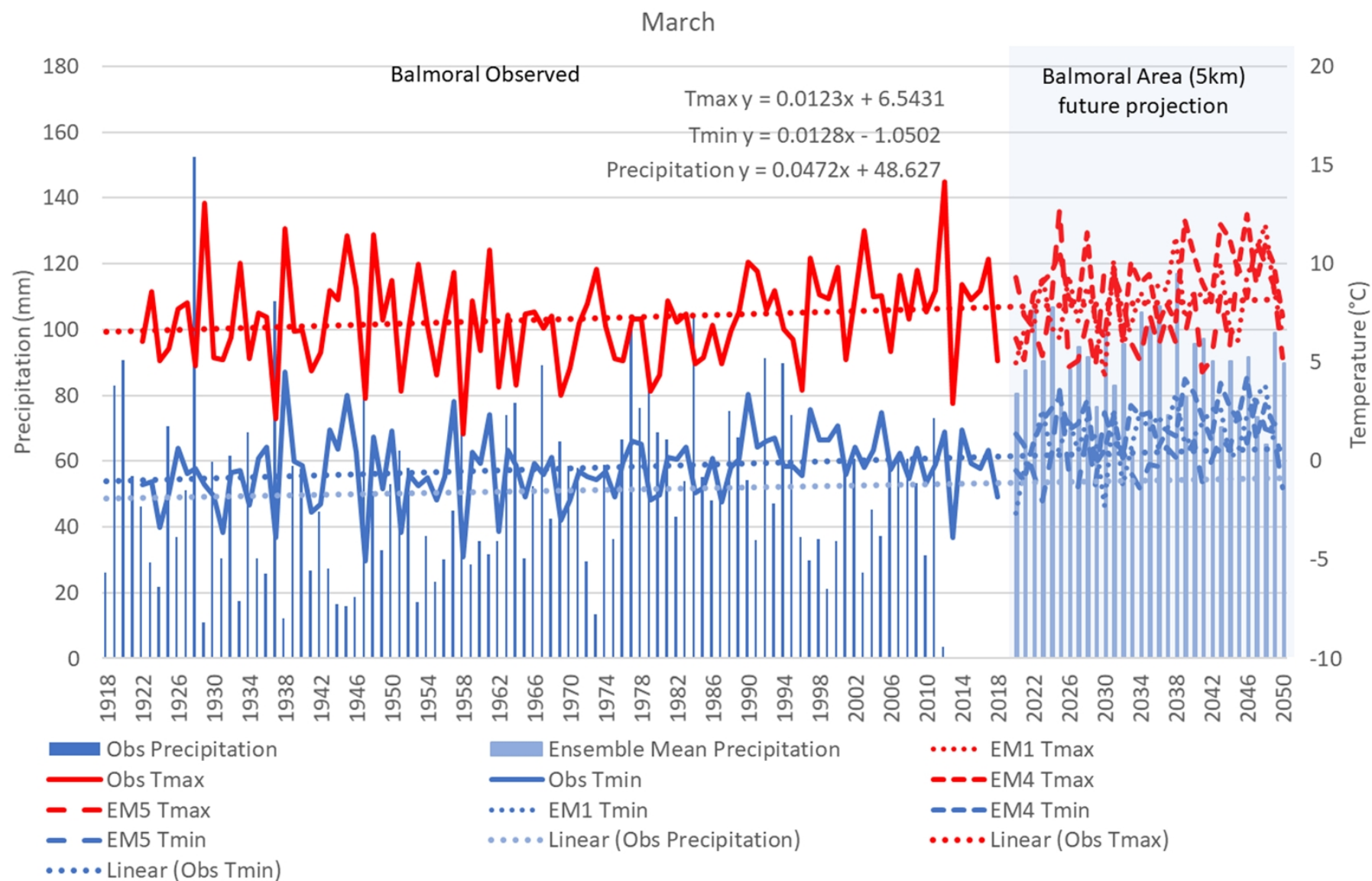
Figure 10: Weather data trends for March, Balmoral 1918-2018 and estimated future 2020-2050 (RCP8.5)
