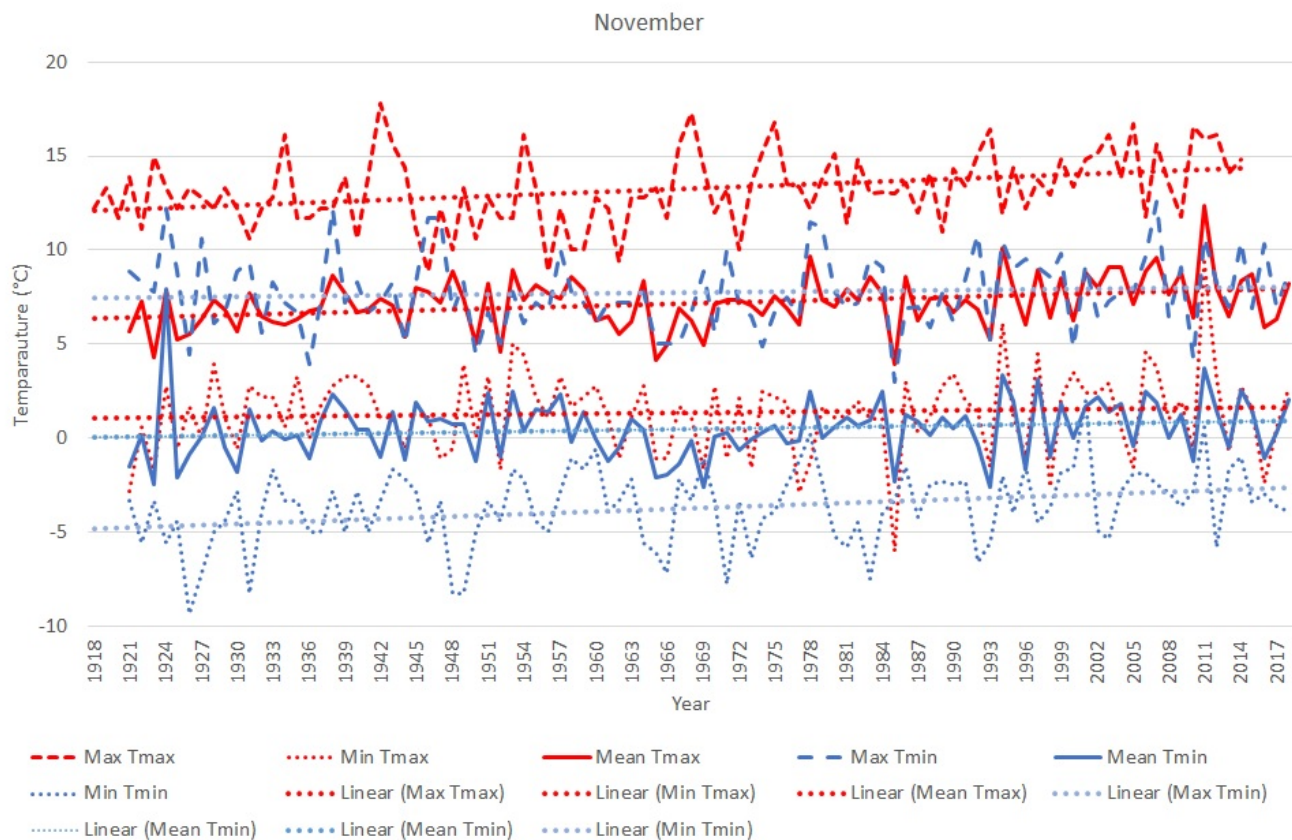
Figure 1: Changes in Balmoral's highest and lowest values of daily maximum and minimum air temperature and estimated trends for November.
