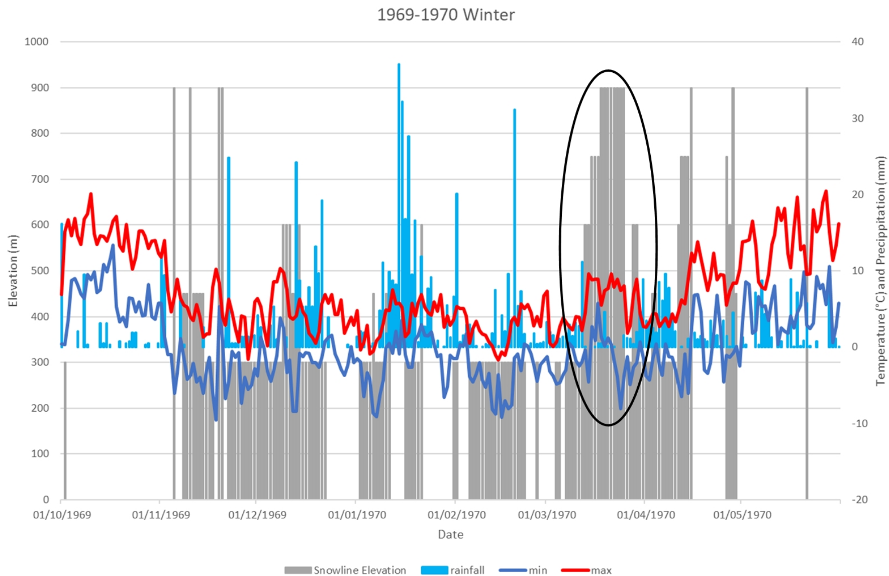
Figure 13: Relationship between maximum and minimum temperature and precipitation with snow cover elevation, Whitehillocks 1969-70.
