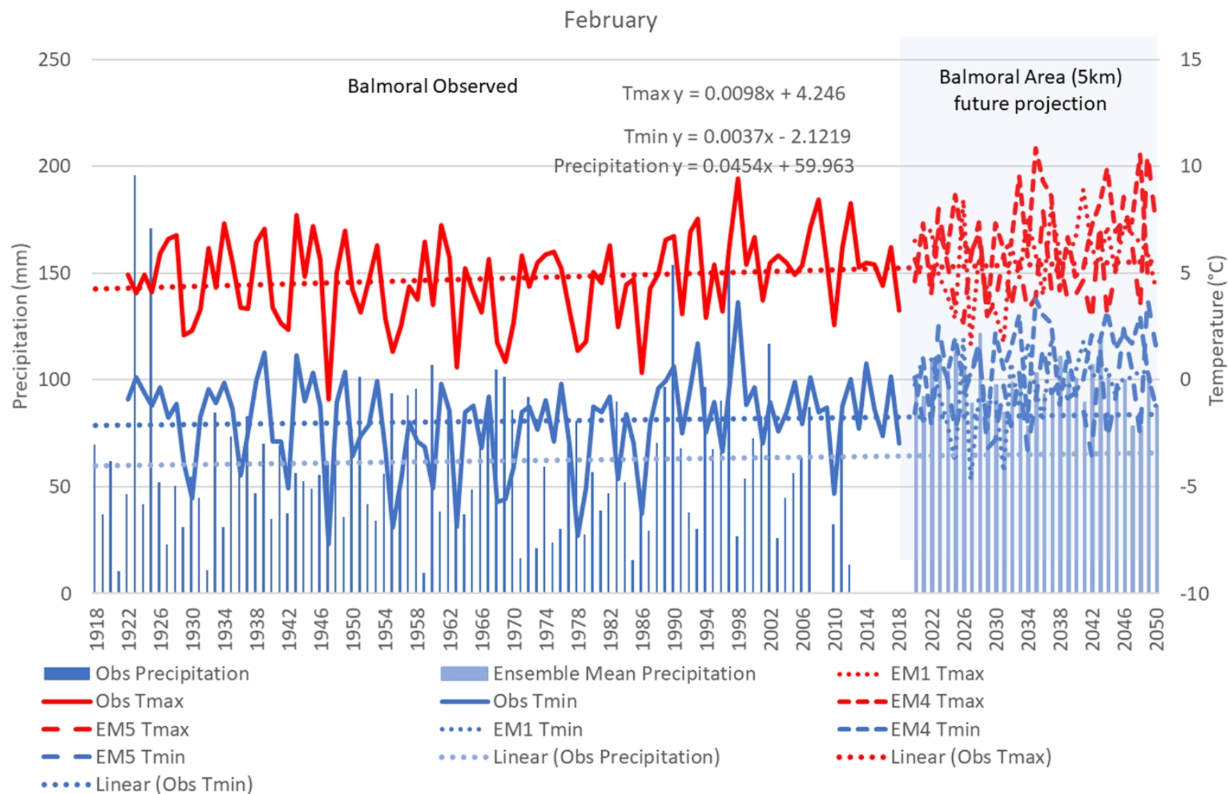
Figure 9: Weather data trends for February, Balmoral 1918-2018 and estimated future 2020-2050 (RCP8.5)
