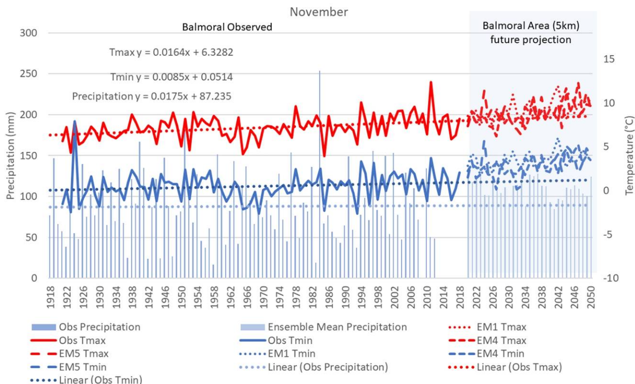
Figure 3: Weather data trends for November, mean monthly maximum and minimum temperature and total precipitation for Balmoral 1918-2018 and estimated future 2020-2050 projection (RCP8.5)
