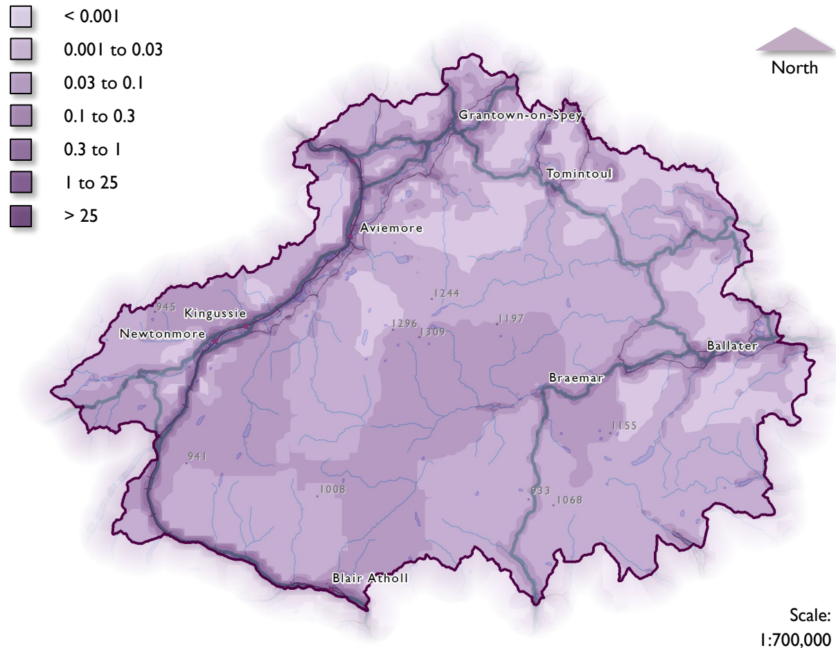
Figure 21 Emissions of Nitrogen Oxides (NO x ) as NO 2 in tonnes in the Cairngorms National Park in 2015.
